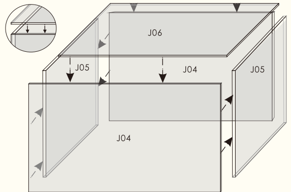
scale 1:6 J04 Transparent cover 25*21*0.15cm 2pieces
